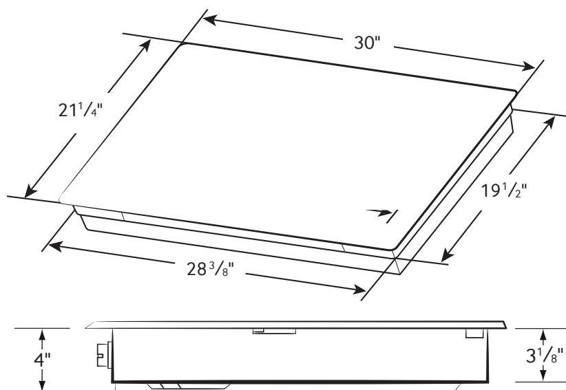
Cooktop Dimensions
